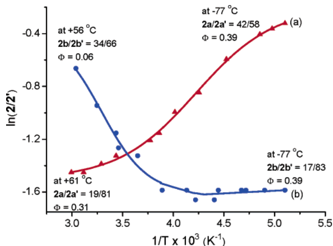
FIGURE 5. Eyring plots of regioselectivity, \ln(2/2') , against 1/T ( K^{-1} ) in the Paternò–Büchi reaction of (a) red triangles, 2-methylfuran ( 2a ) and (b) blue circles, 3-methylfuran ( 2b ) with benzophenone.
