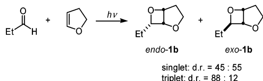
Scheme 10. Diastereoselectivity as an Indicator for Triplet versus Singlet Process
