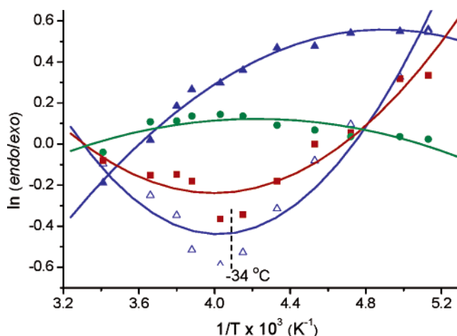
FIGURE 8. Eyring plots for photocycloaddition to 2,3-dihydrofuran at different substrate concentrations: (a) propionaldehyde, ( \blacktriangle ) 1.0 M, ( \triangle ) 5.0 M; (b) acetaldehyde, ( \blacksquare ) 1.0 M; (c) isobutyraldehyde, ( \bullet ) 1.0 M.
